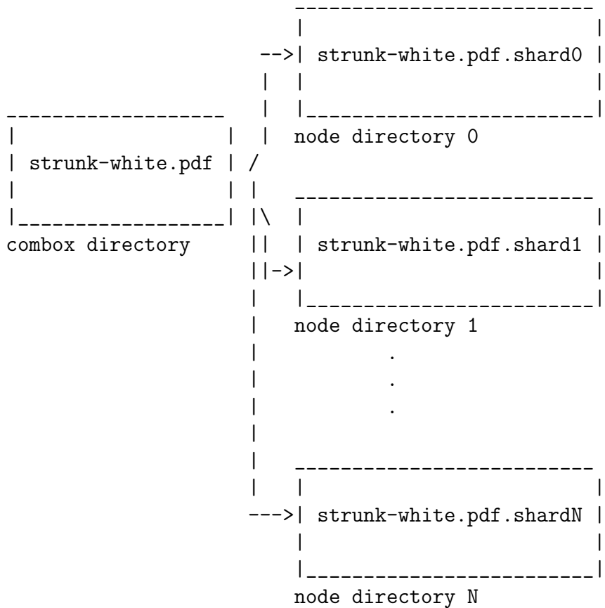
Figure 1-1: combox overview - Splitting a file in the combox directory and spreading it across N node directories.
