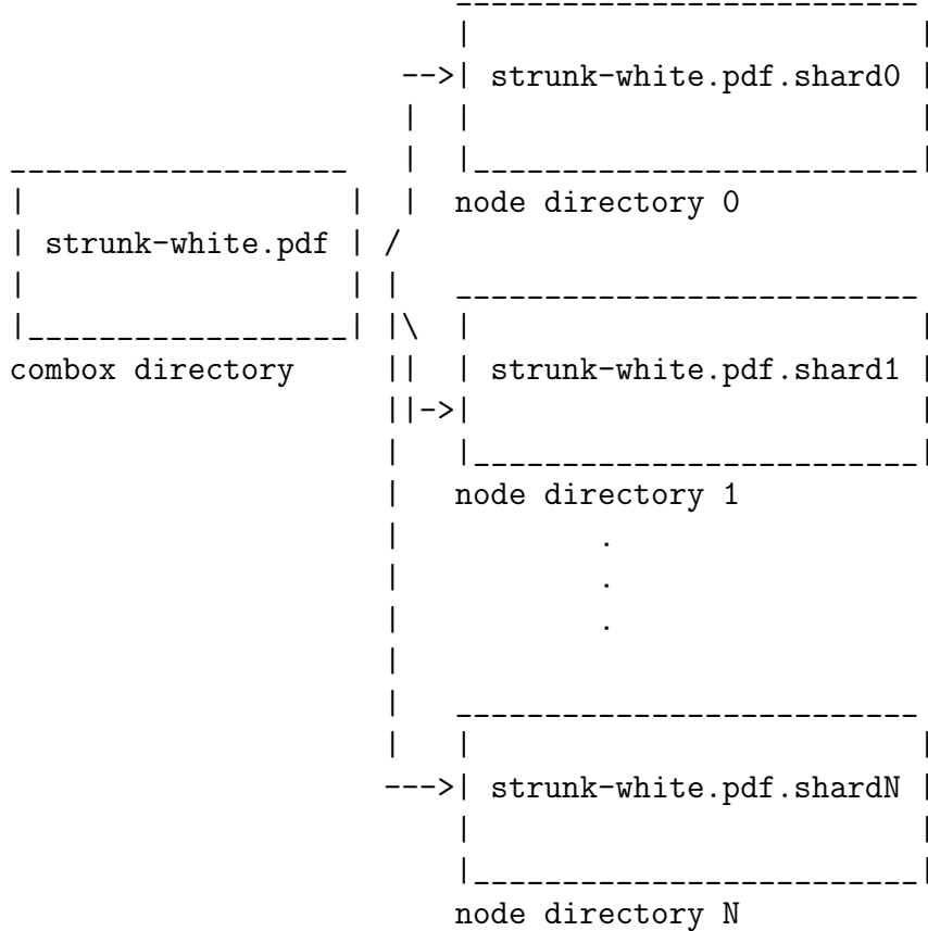
Figure 1-1: combox overview - Splitting a file and spreading it across N node directories.
